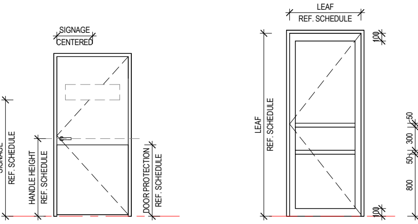
DOOR DIMENSION DIAGRAM APPLIES TO LEAF TYPES A1-8, C2-4, FS-11 LEAF TYPE D1 LEAF TYPE D2 AS ABOVE, WITHOUT MID RAILS
